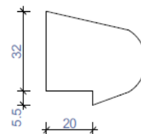
VENT Over Fascia Vent - G2500I
