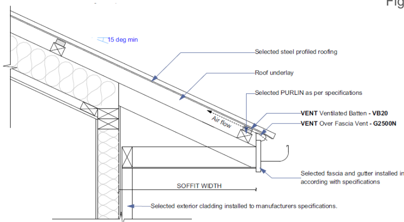
Fig C: Skillion Roof Application
